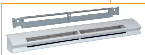
MORTICE carried out on the window frame: Double slot: 2 x (172 x 12) mm
